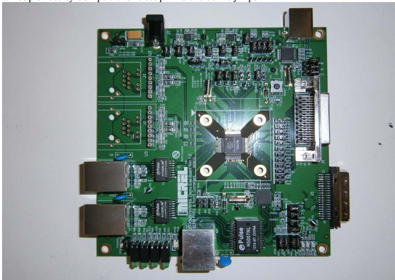
Figure 1 KSZ8765CLX-EVAL Board
